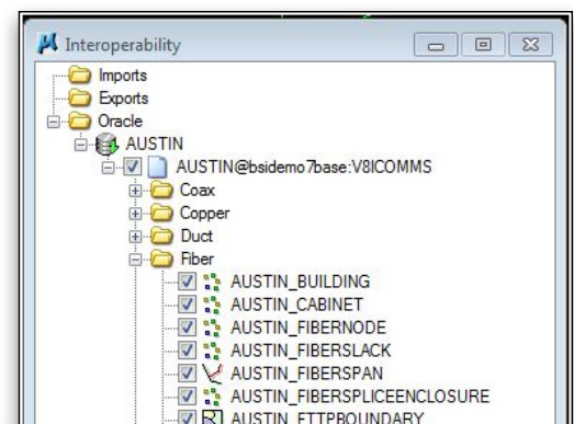
The interoperability dialog allows users to select and extract only the network components that need to be modified during their work session.
