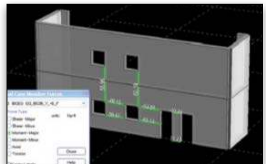
Shear wall forces displayed at any cross section.
